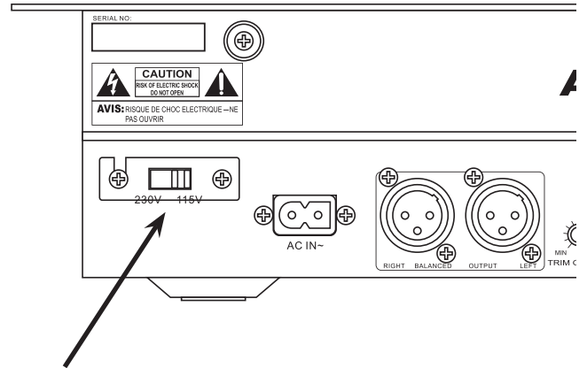
VOLTAGE SELECTOR SWITCH
